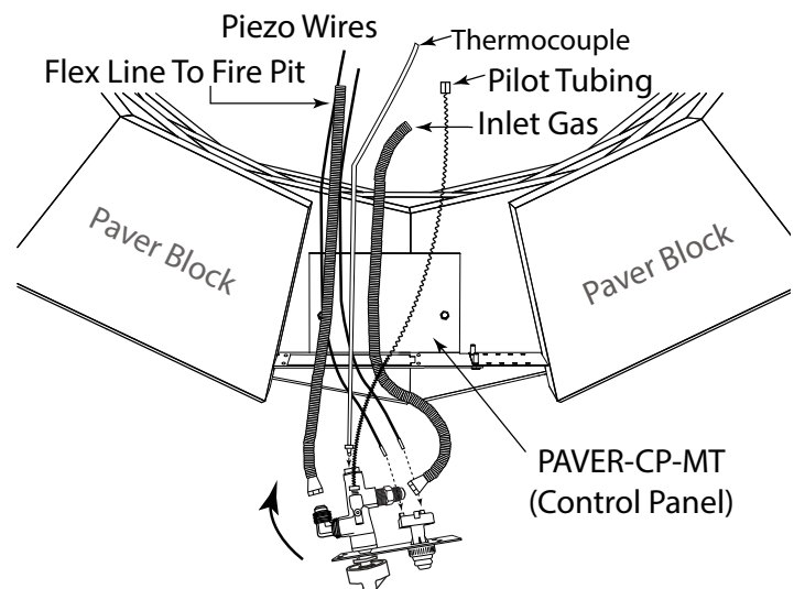
Fig. 5 Installing control panel into PAVER-CP-MT mounting plate.
