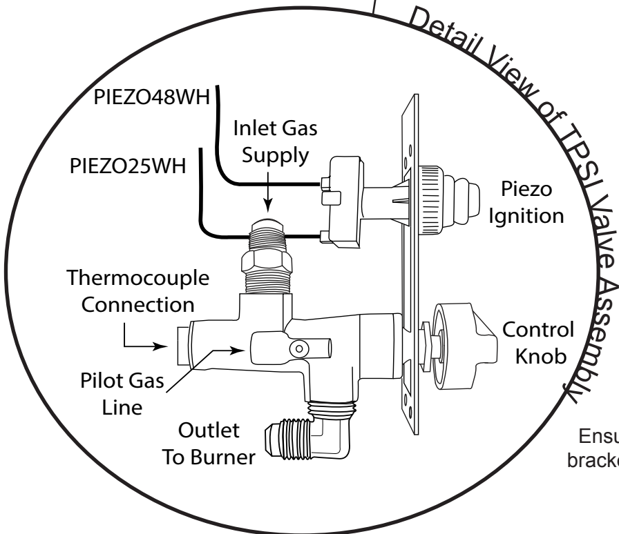
Fig. 13 Typical installation.
