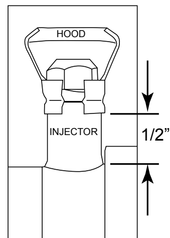
Fig. 12 Shows 1/2” spacing from bottom of injector.
